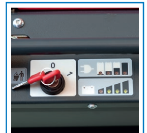
Battery and onboard charger display including excessive discharge protection
