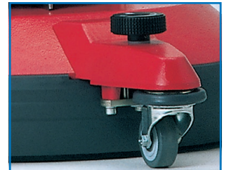
Guide wheel with brush-pressure adjusting screw
