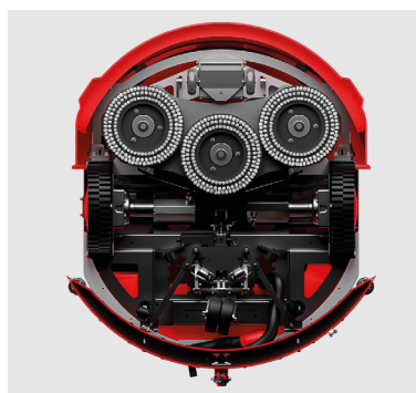
Optimal brush layout
